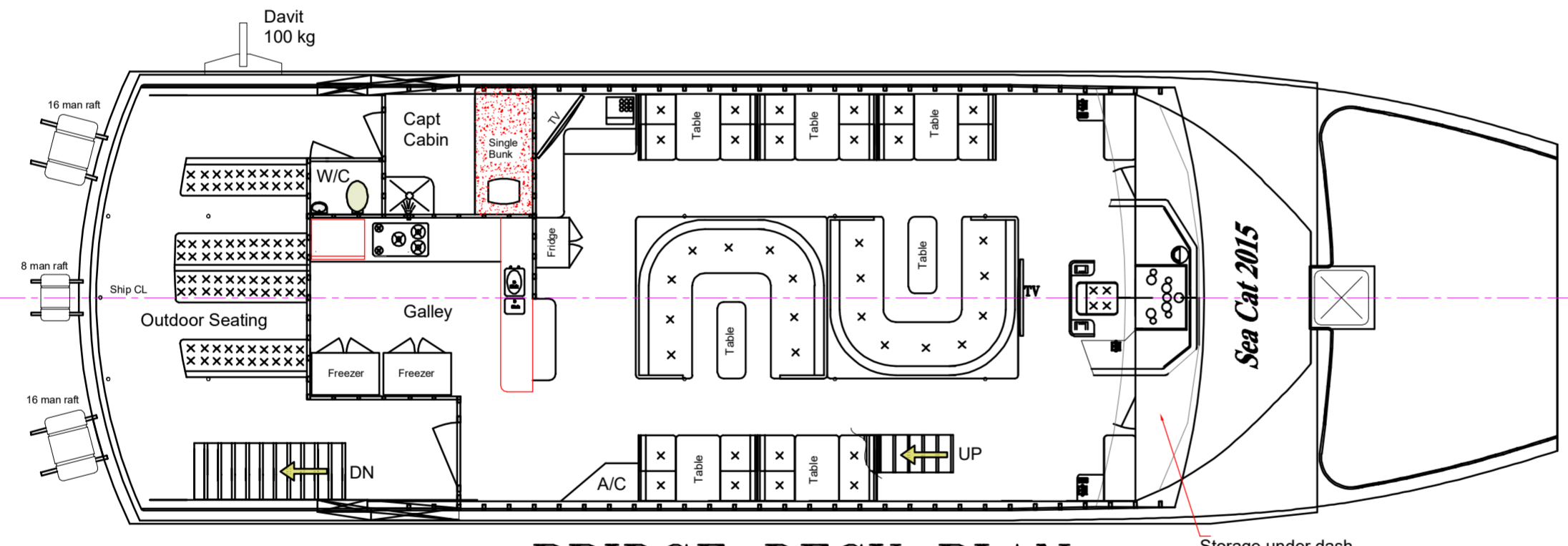
BRIDGE DECK PLAN
