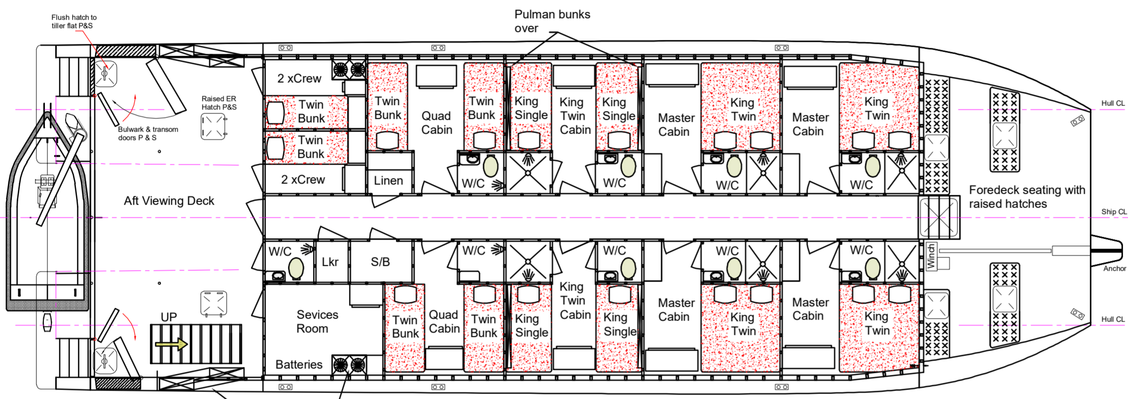
MAIN DECK PLAN
