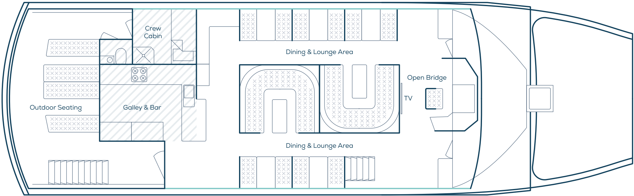
BRIDGE DECK
