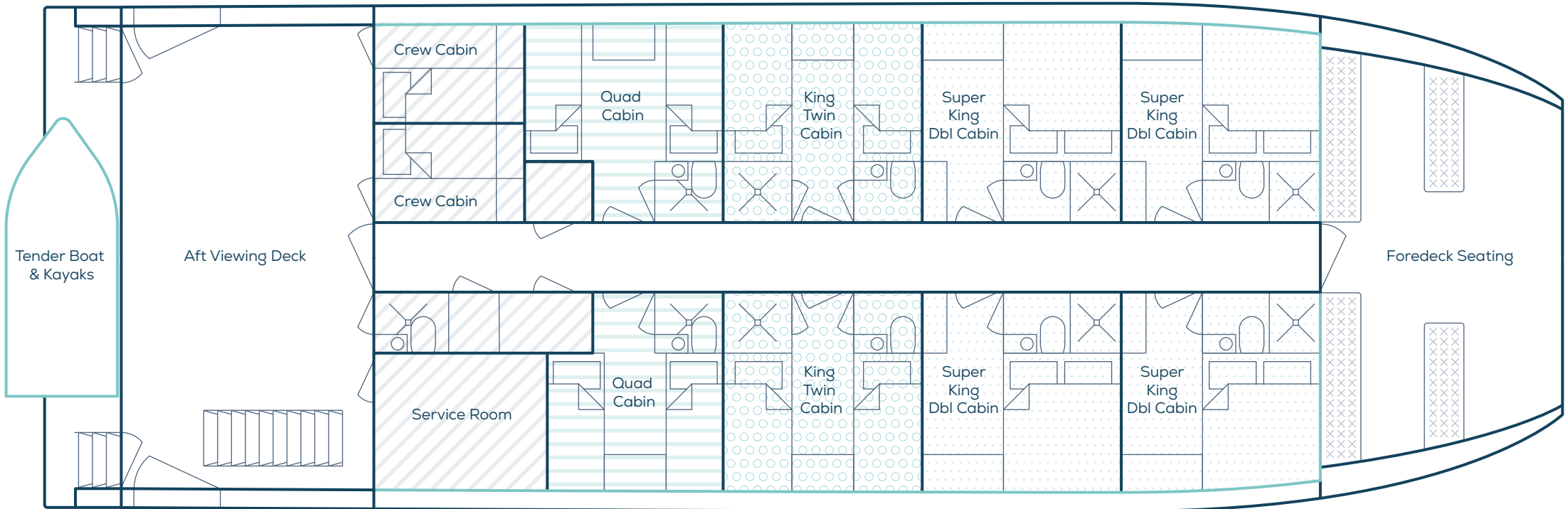
MAIN DECK
